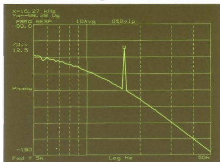
Figure 3-4: One-decade frequency response phase
